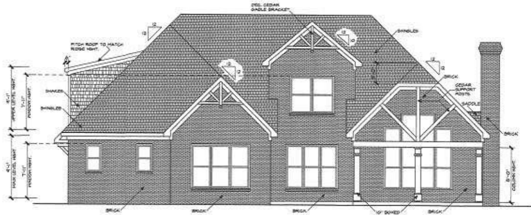
REAR ELEVATION
