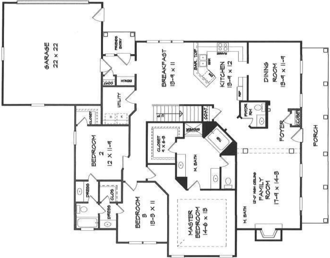
FLOOR PLAN
