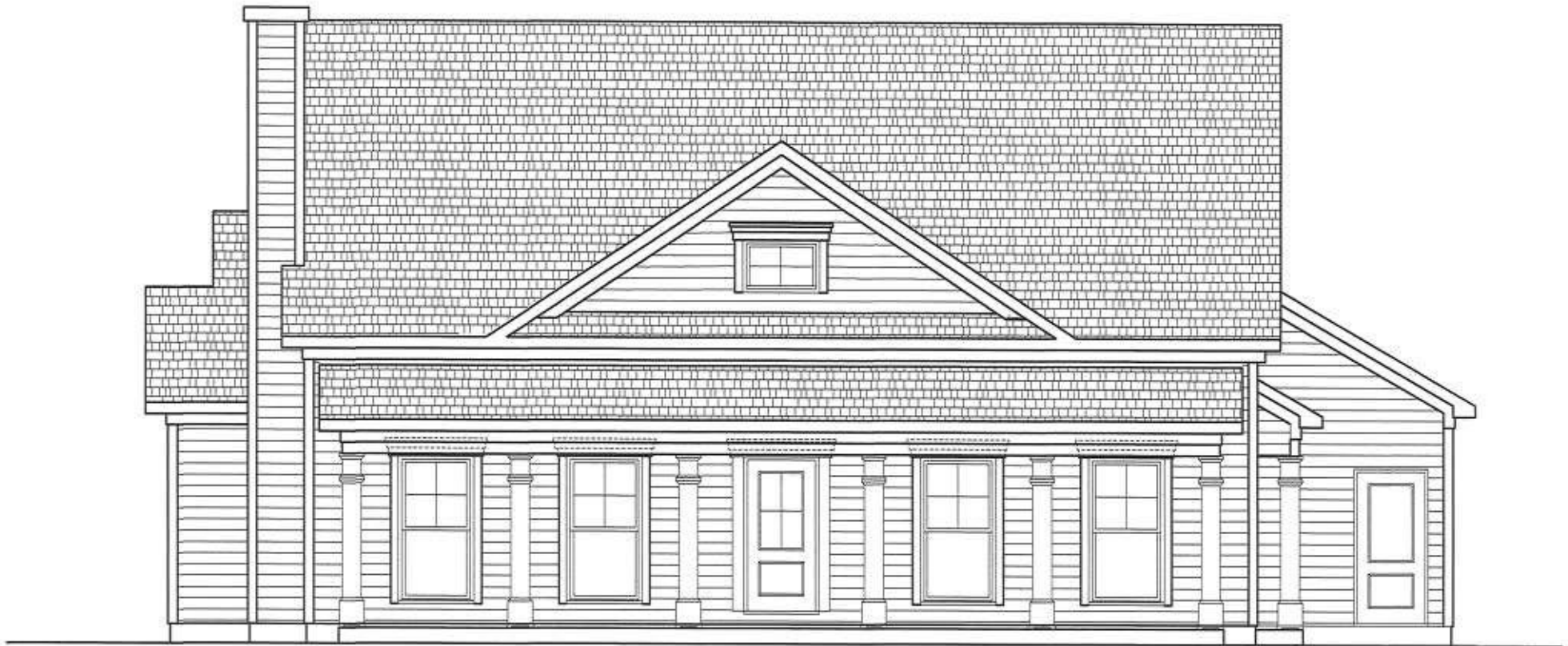
FRONT ELEVATION
